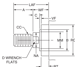
Thread Style 2 Intermediate Male
