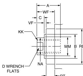
Thread Style 3 Short Female
