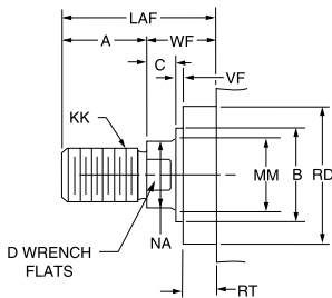
Thread Style 1 Small Male
