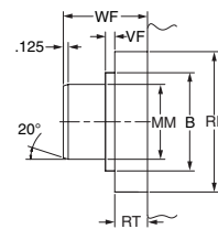
Style 6 Stub End
