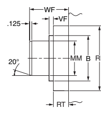
Style 6 Stub End
